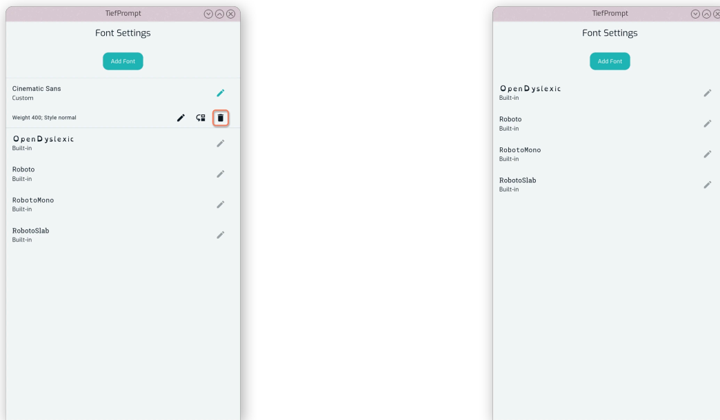
Figure 39: “Delete Variant” highlighted, with last variant of a font family being deleted Lastly, by pressing the edit icon next to a font variant, you can edit the variant’s weight and whether it is an italic font or not. This is useful if the app does not detect the variant correctly, or if you want to change the weight of a font variant.
